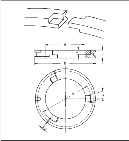
With overlapped mortise joint for shaft seal YFZ 54502
