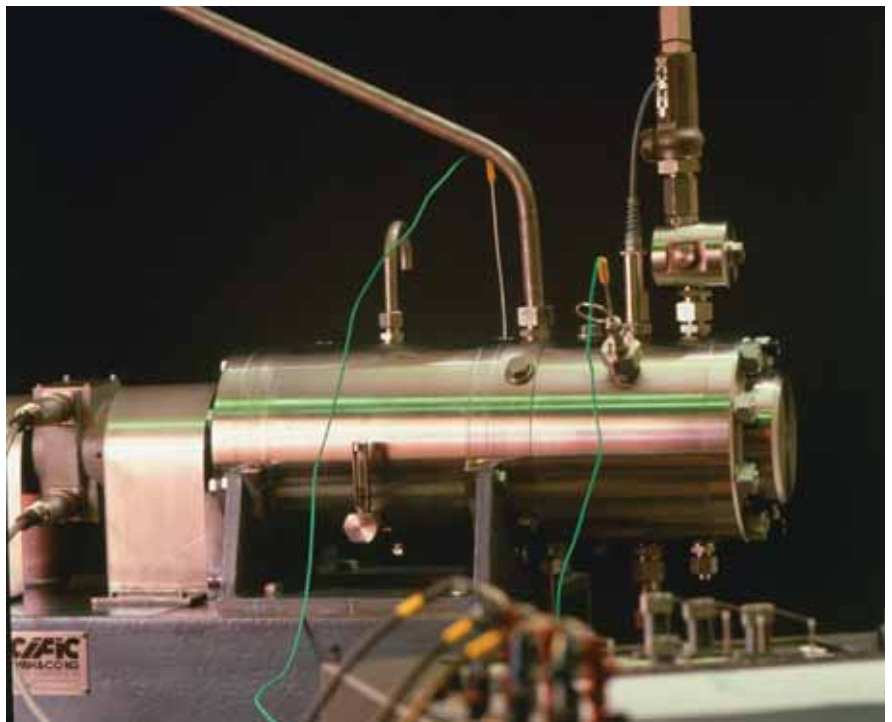
Testing stand for blister tests with high viscosity oils as the medium to be sealed off
