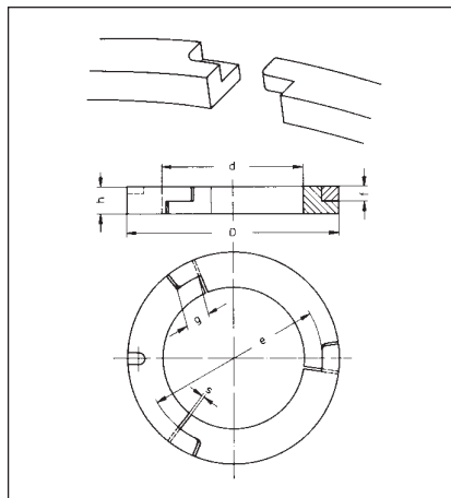
With overlapped mortise joint for piston seal YFZ 54504
